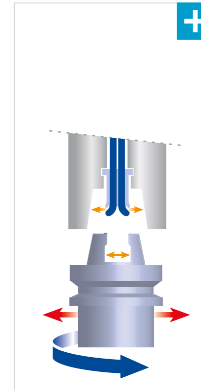
HSK shank
