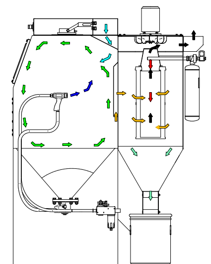
▼ Injector blast principle
